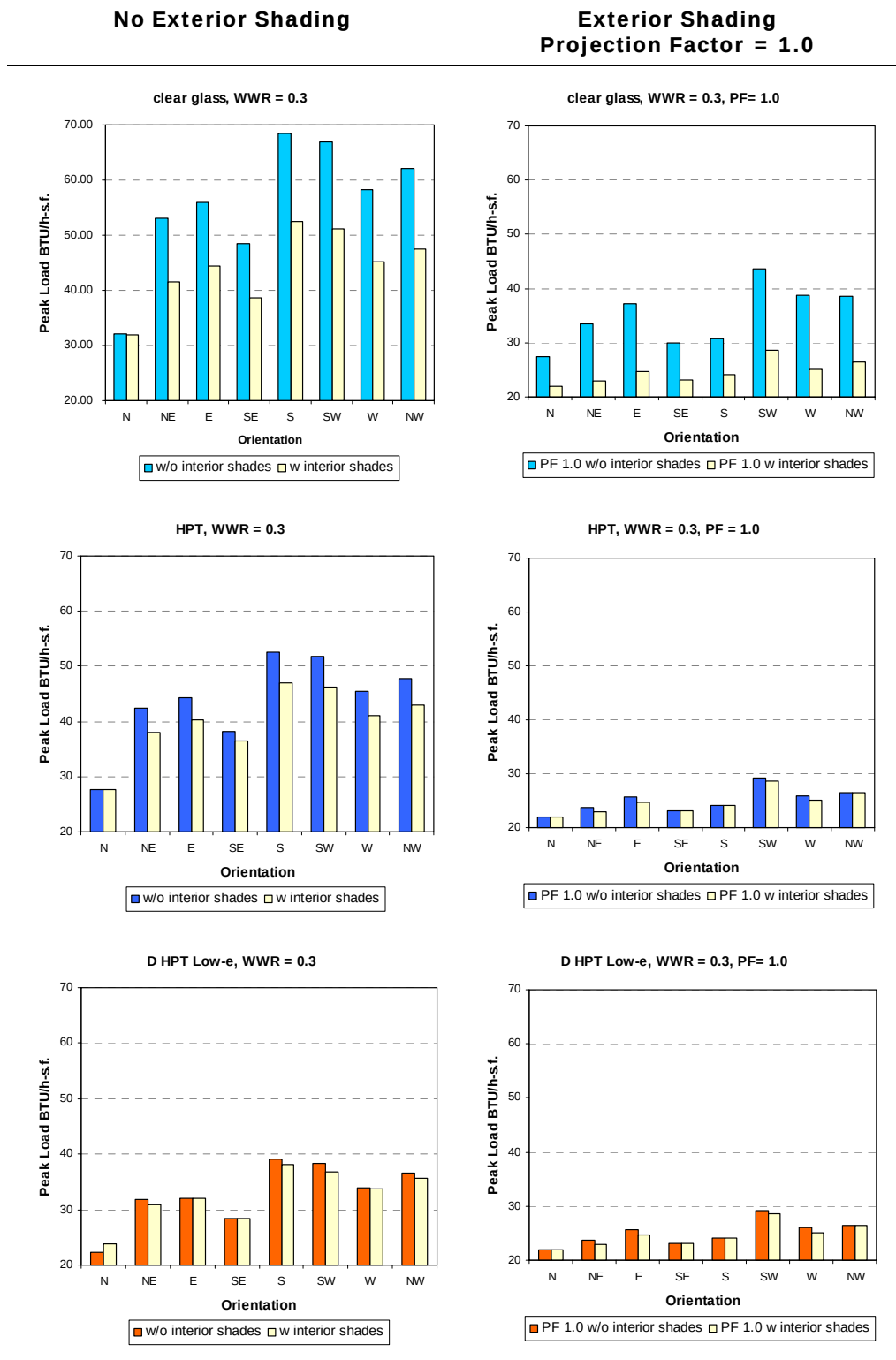
Figure 5-8. Effect of interior shades on peak cooling load . WWR = 0.30. Graphs on the left show windows without exterior shading, while graphs on the right show windows that have overhangs with a projection factor of 1.0.
