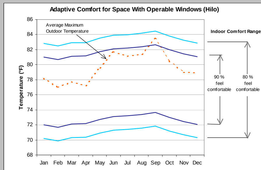
Figure 2-3. Indoor comfort range in naturally ventilated buildings in Hilo (based on comfort model shown in Figure 2-1).
