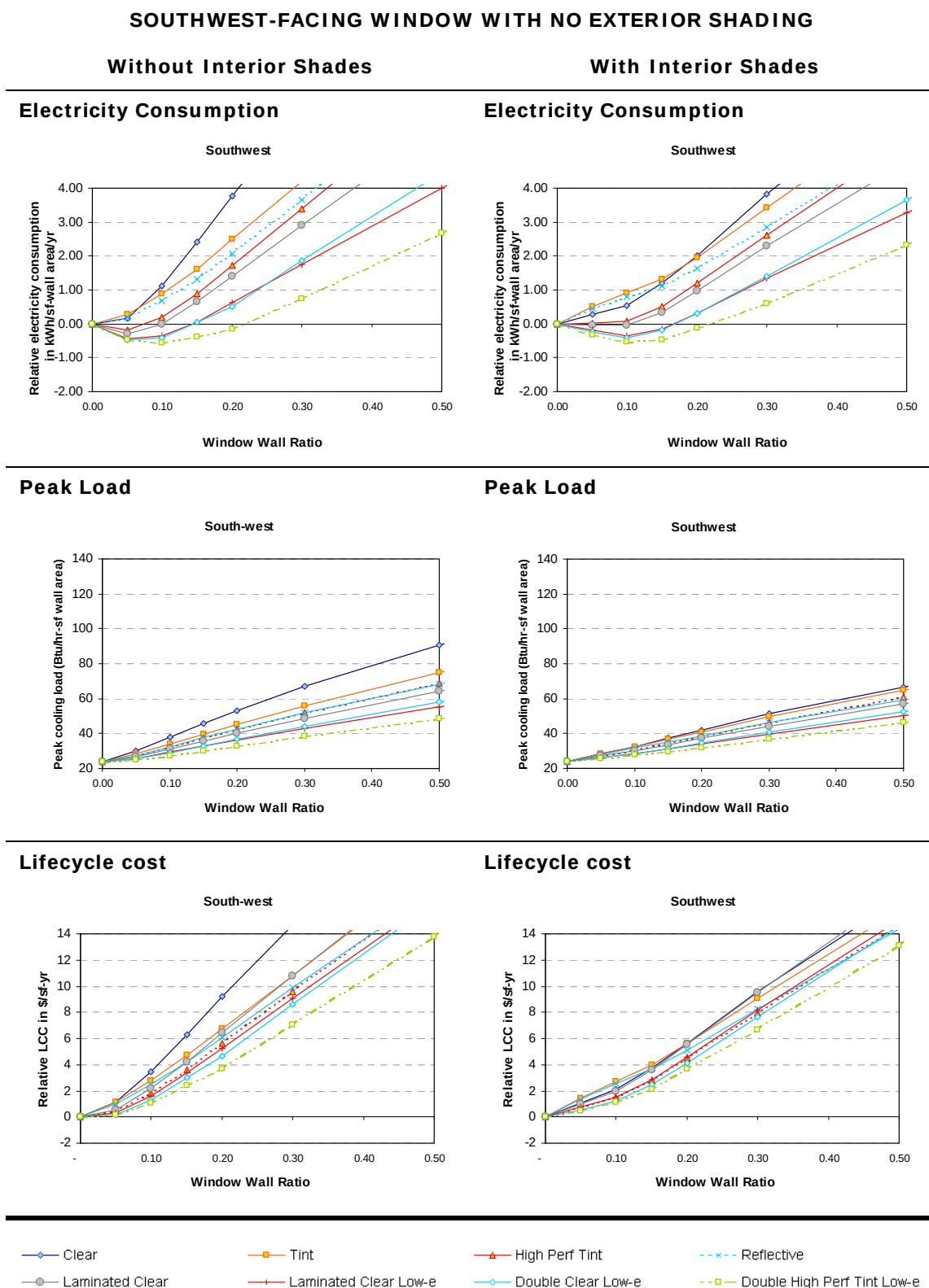
Figure 5-54. Southwest window, no overhang. Impact of WWR on electricity consumption, peak cooling load, and lifecycle cost, for windows with and without interior shades.
