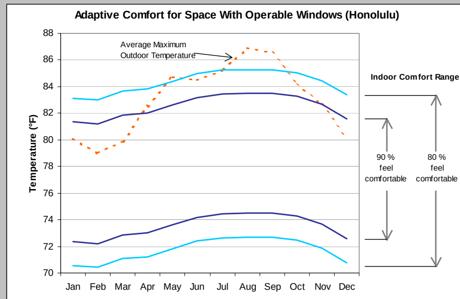
Figure 2-2. Indoor comfort range in naturally ventilated buildings in Honolulu (based on comfort model shown in Figure 2-1).
