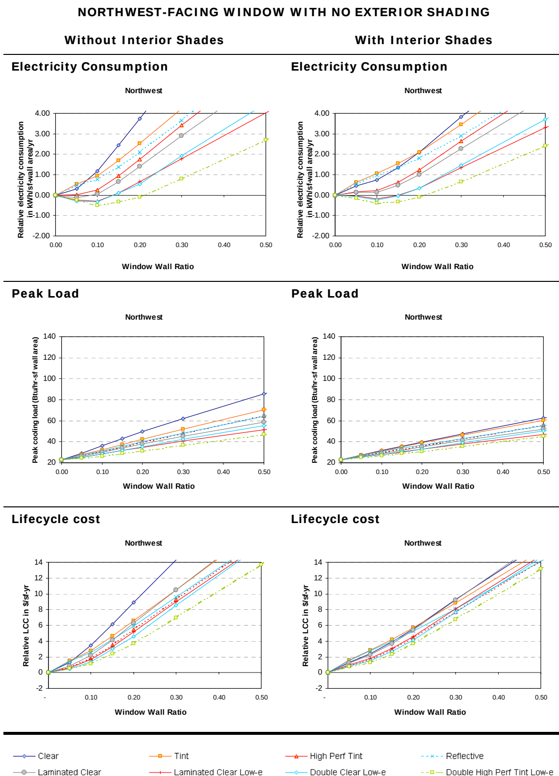
Figure 5-62. Northwest window, no overhang. Impact of WWR on electricity consumption, peak cooling load, and lifecycle cost, for windows with and without interior shades.
