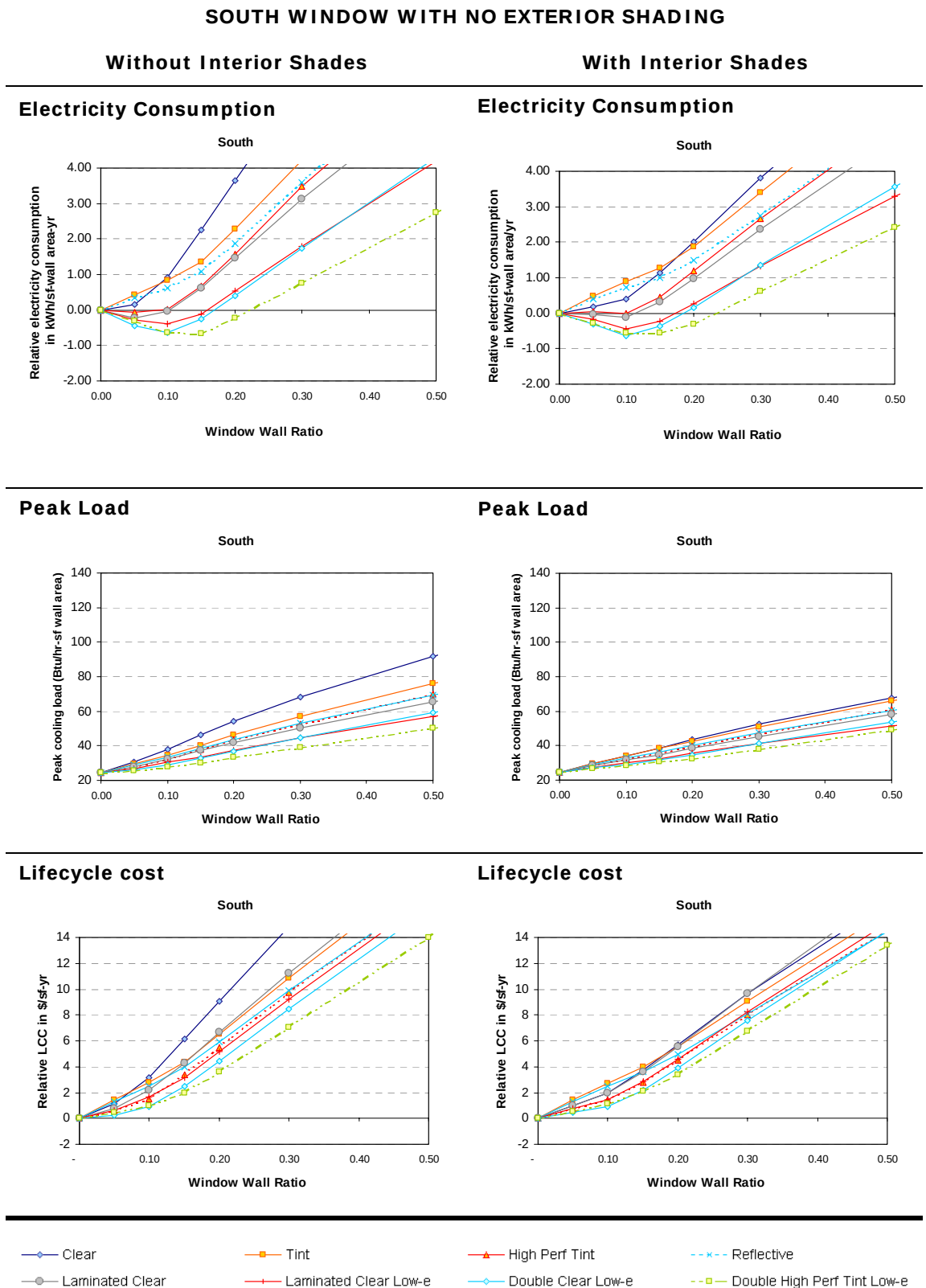
Figure 5-12. Impact of WWR on electricity consumption, peak cooling load, and lifecycle cost, for windows with and without interior shades. South-facing window only (see the Windows Performance Data section for other orientations).
